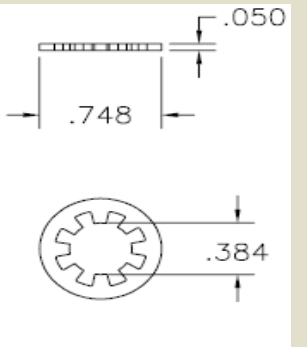
P/N 1000798 3/8 shake proof washer
