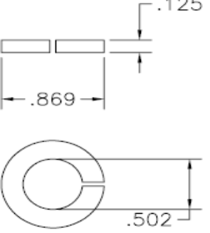
P/N 1000786 1/2 lock washer
