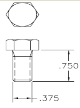
P/N 1000663 MS 3/8 x 3/4
