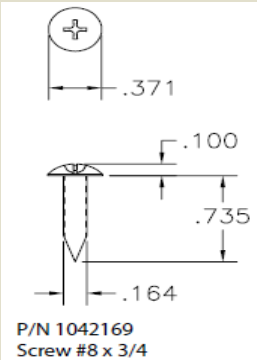
P/N 1042169 Screw #8 x 3/4
