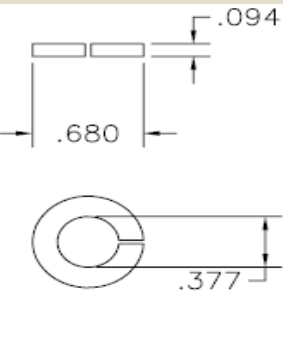
P/N 1000781 3/8 lock washer
