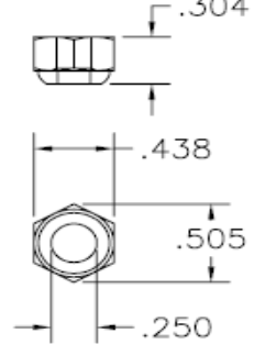
P/N 1000760 1/4 lock Nut
