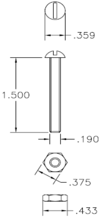
P/N 1000702 Stove bolt 3/16 X 1 1/2
