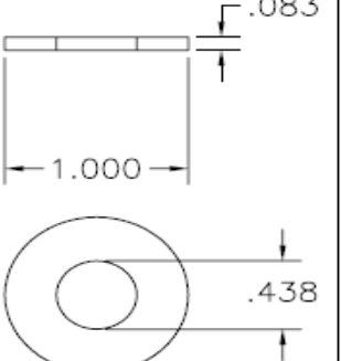
P/N 1000784 3/8 flat washer
