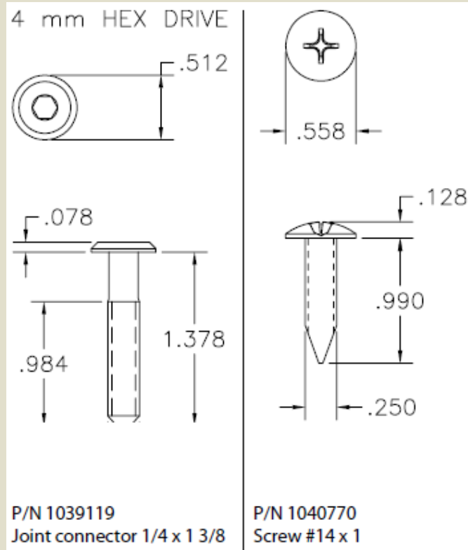
1039119 Joint Connector 1/4x1 3/8
